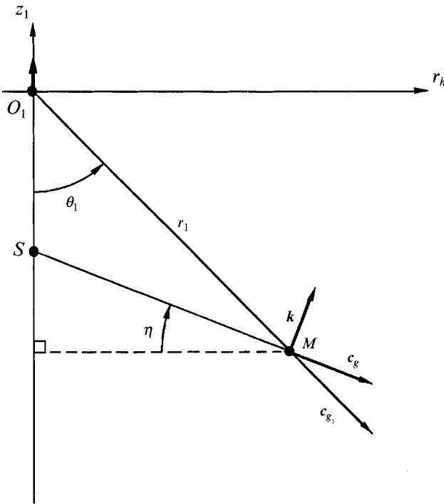
FIGURE 10. Geometry for internal wave radiation by a steady source in uniform vertical motion.
